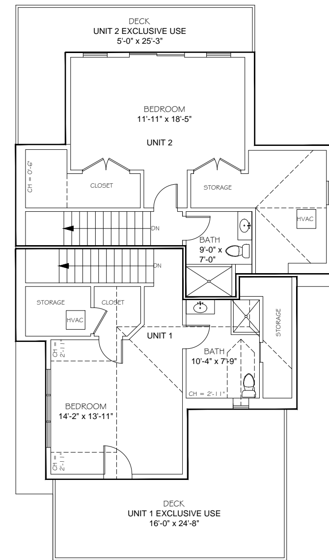
THIRD FLOOR PLAN Ceiling Height = 9'-8"
