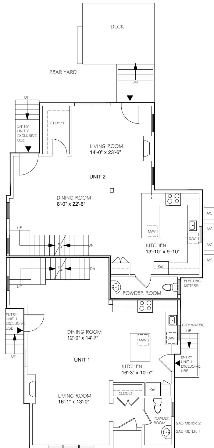
FIRST FLOOR PLAN Ceiling Height = 9'-3"
