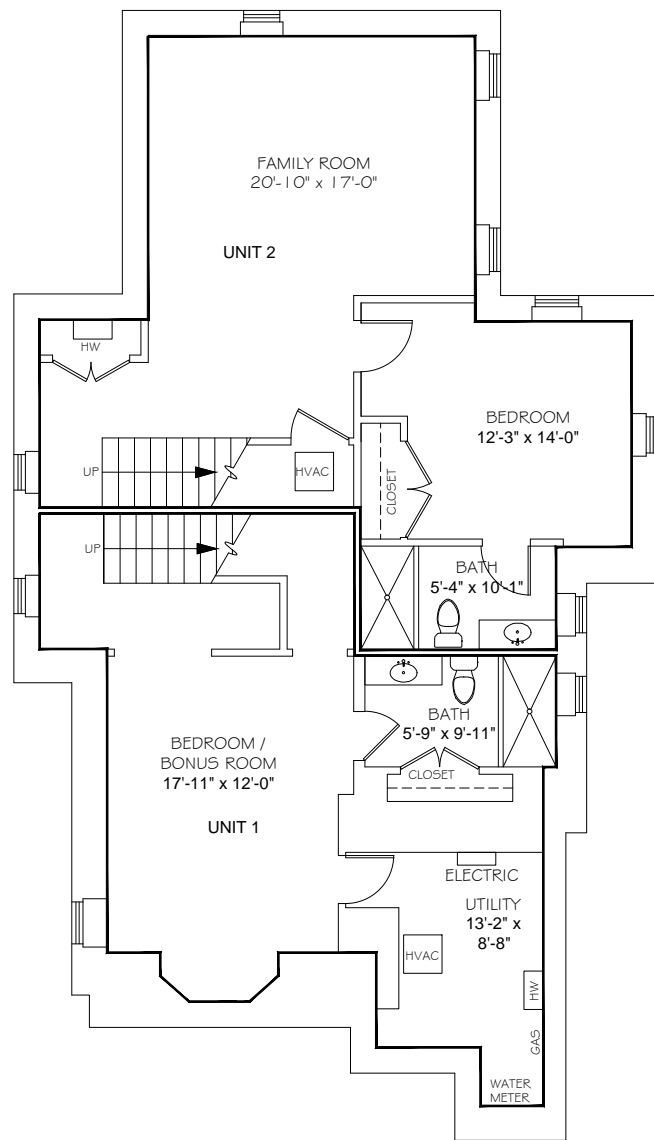
LOWER LEVEL PLAN Ceiling Height = 8'-0"
